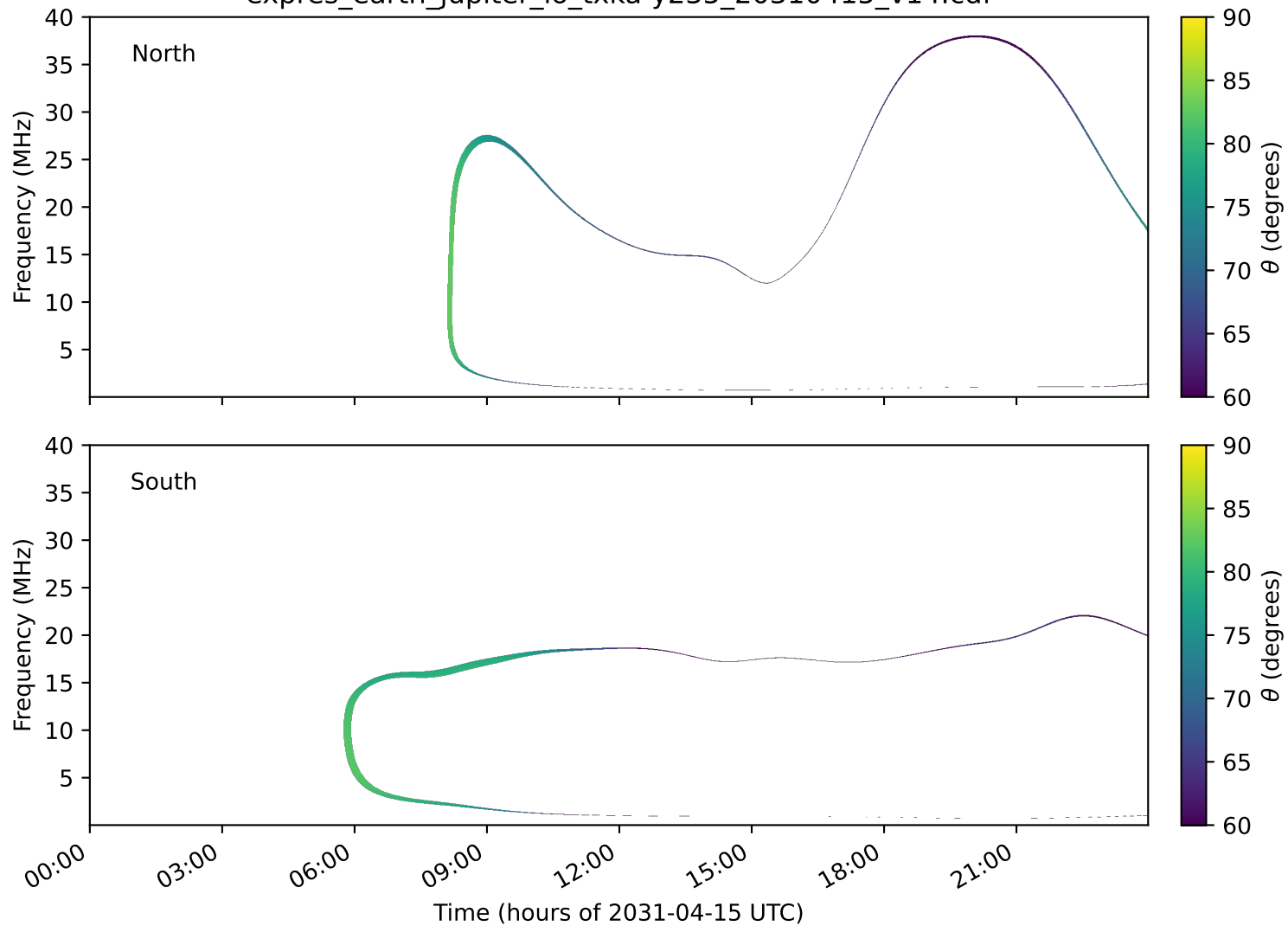
expres_earth_jupiter_io_txka-y235_20310415_v14.cdf
