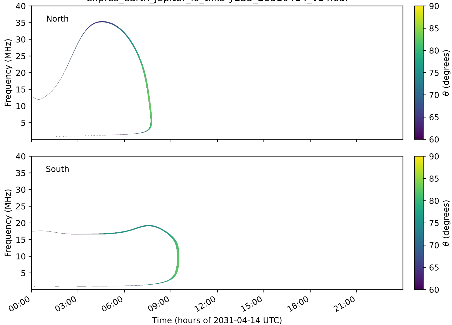
expres_earth_jupiter_io_txka-y235_20310414_v14.cdf
