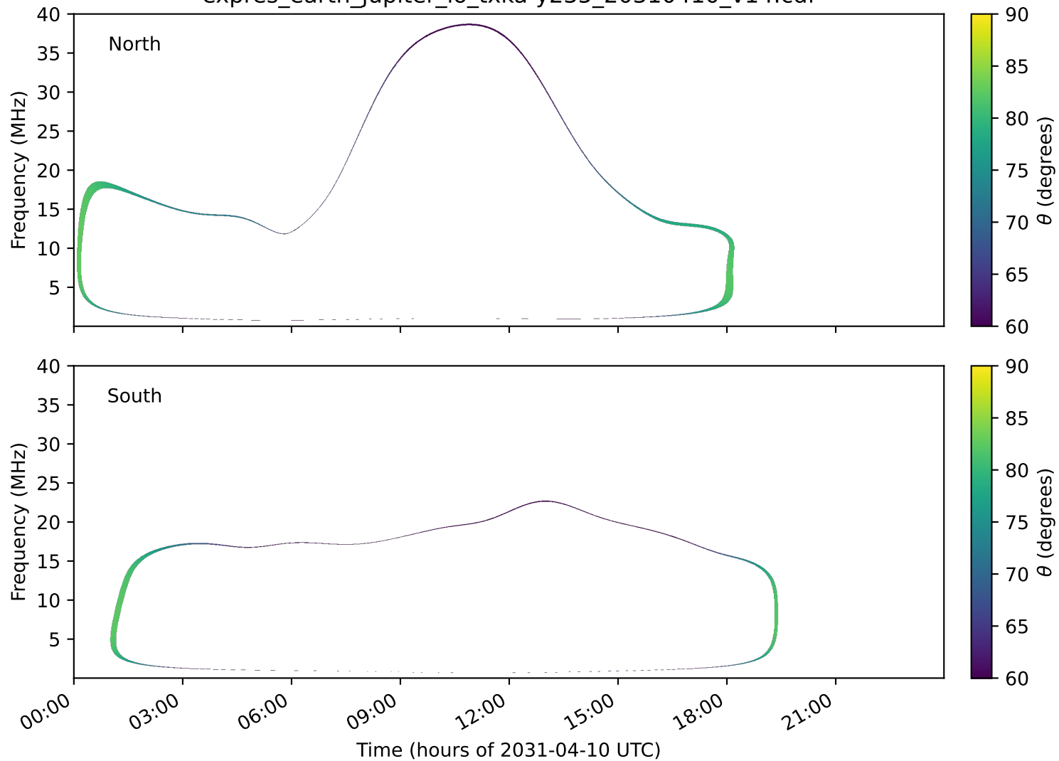
expres_earth_jupiter_io_txka-y235_20310410_v14.cdf
