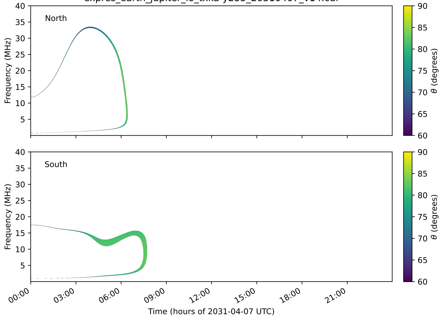
expres_earth_jupiter_io_txka-y235_20310407_v14.cdf
