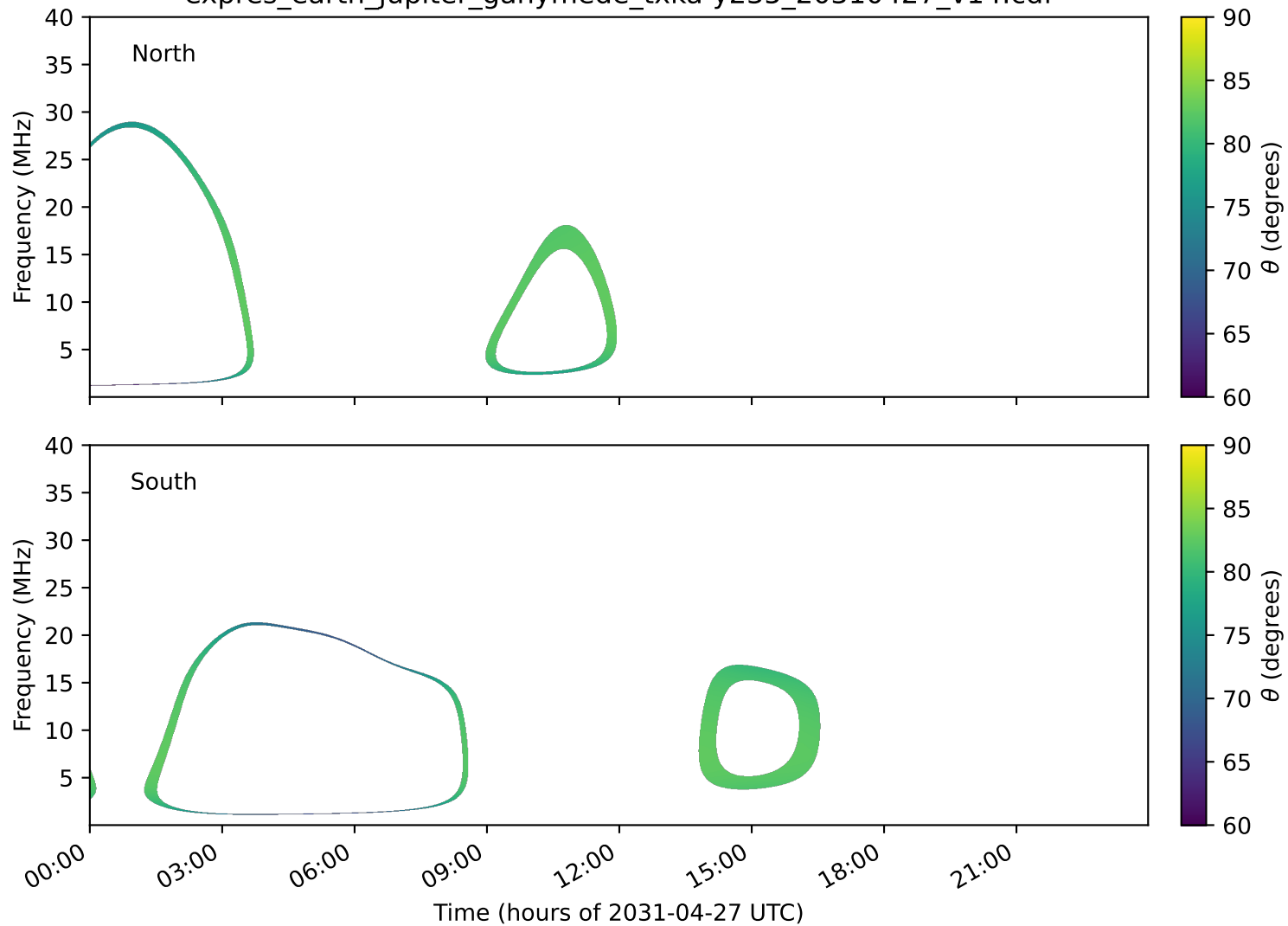
expres_earth_jupiter_ganymede_txka-y235_20310427_v14.cdf
