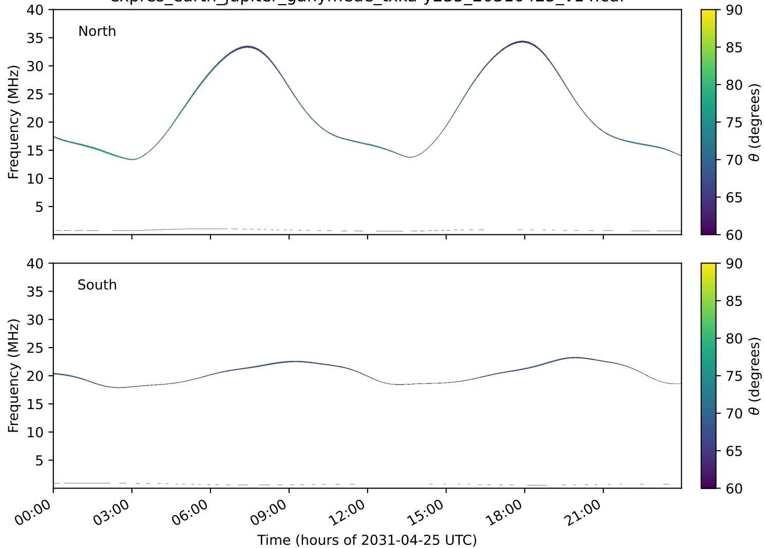
expres_earth_jupiter_ganymede_txka-y235_20310425_v14.cdf
