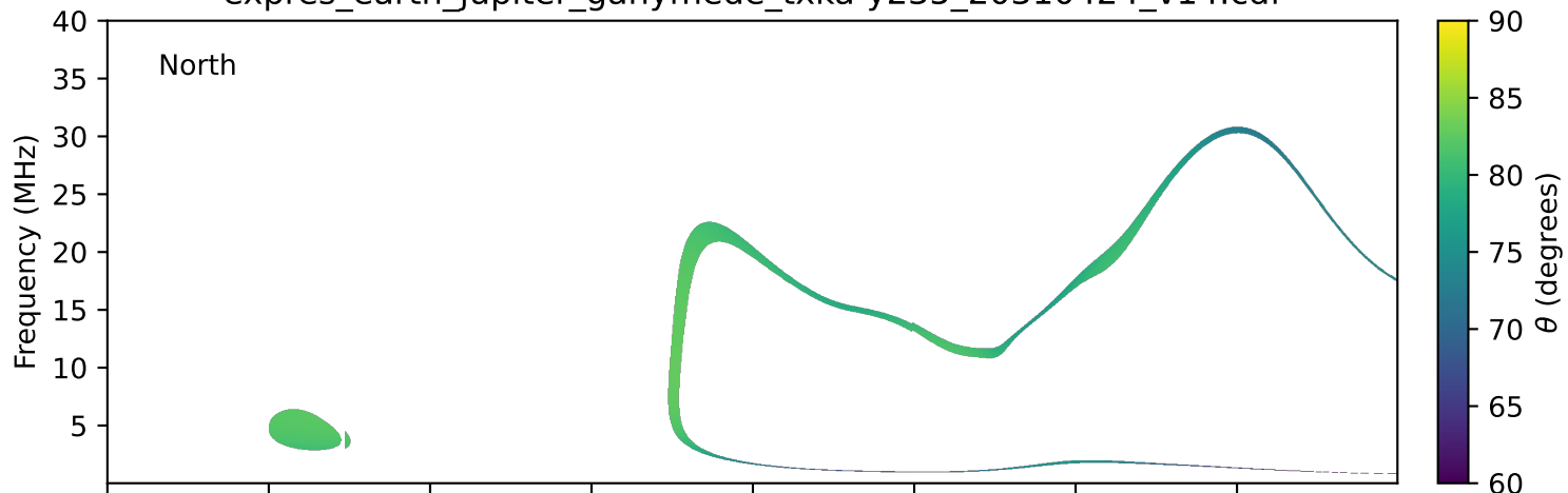
expres_earth_jupiter_ganymede_txka-y235_20310424_v14.cdf
