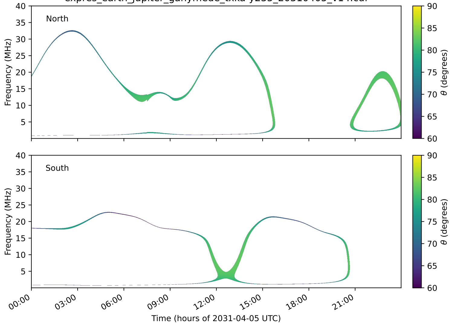
expres_earth_jupiter_ganymede_txka-y235_20310405_v14.cdf
