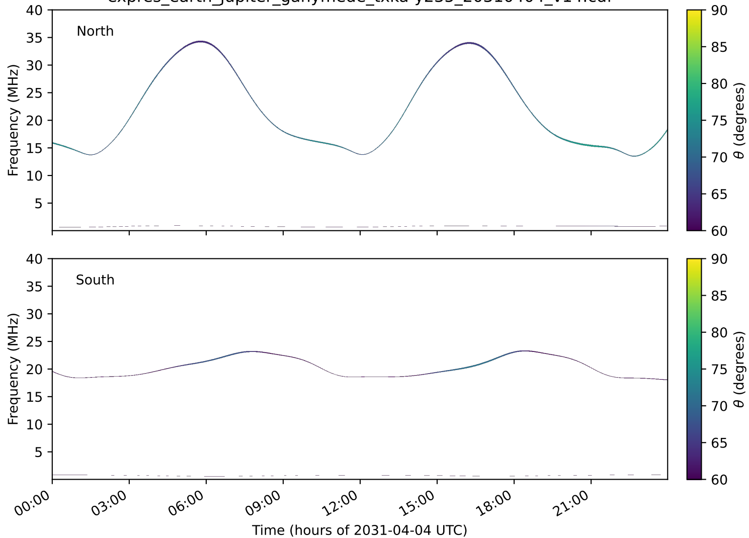
expres_earth_jupiter_ganymede_txka-y235_20310404_v14.cdf
