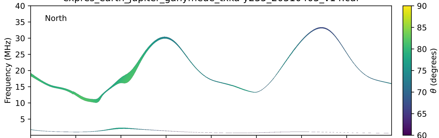
expres_earth_jupiter_ganymede_txka-y235_20310403_v14.cdf
