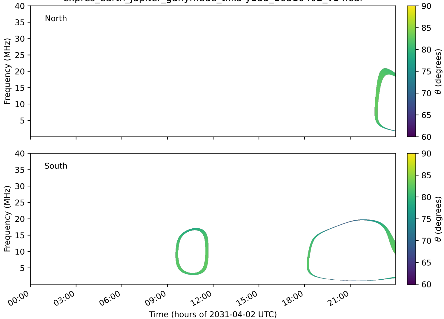
expres_earth_jupiter_ganymede_txka-y235_20310402_v14.cdf
