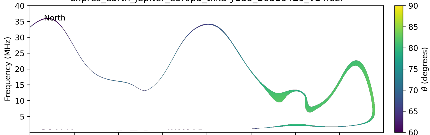
expres_earth_jupiter_europa_txka-y235_20310429_v14.cdf
