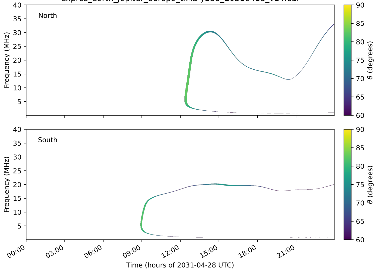
expres_earth_jupiter_europa_txka-y235_20310428_v14.cdf
