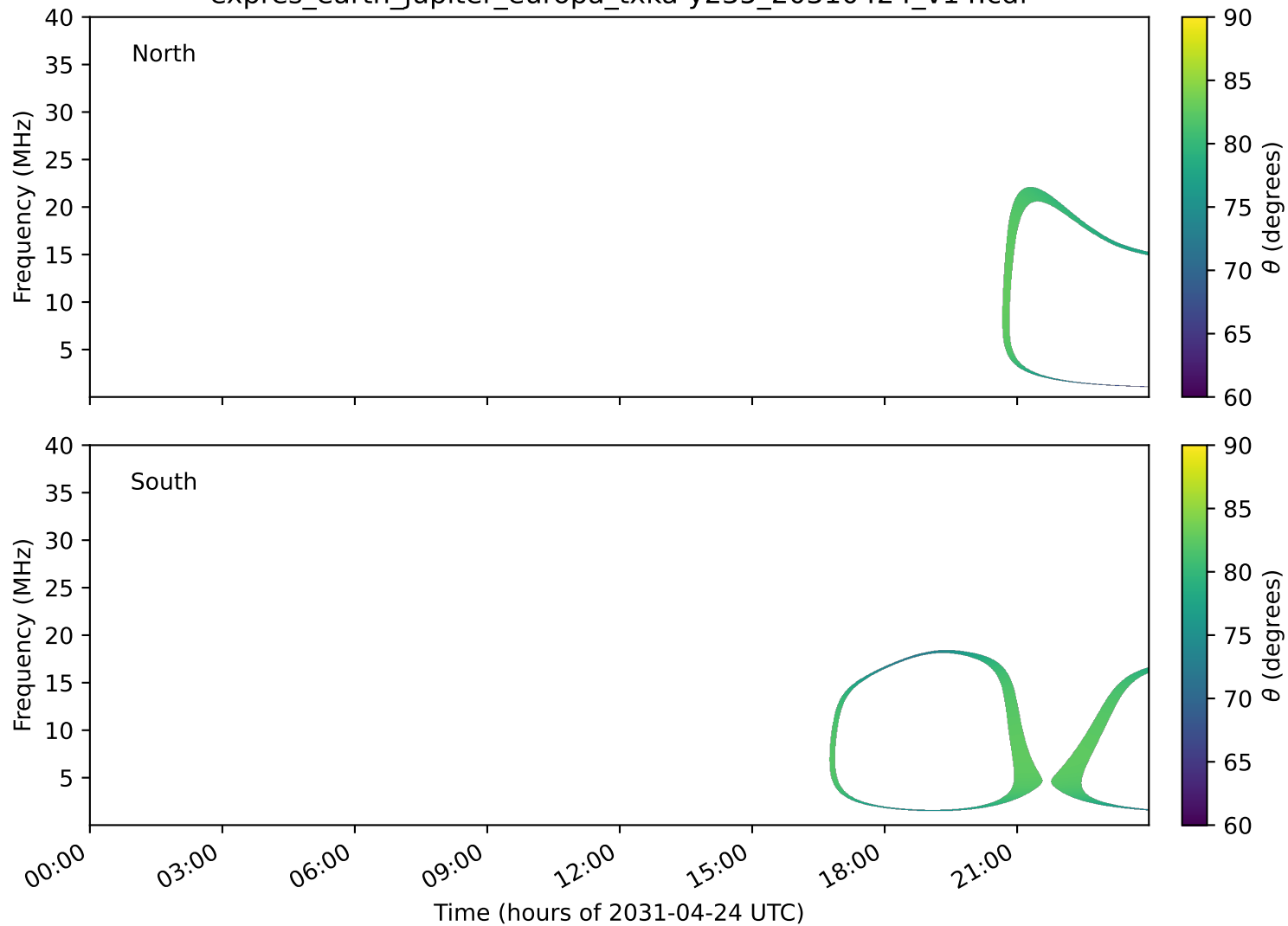
expres_earth_jupiter_europa_txka-y235_20310424_v14.cdf
