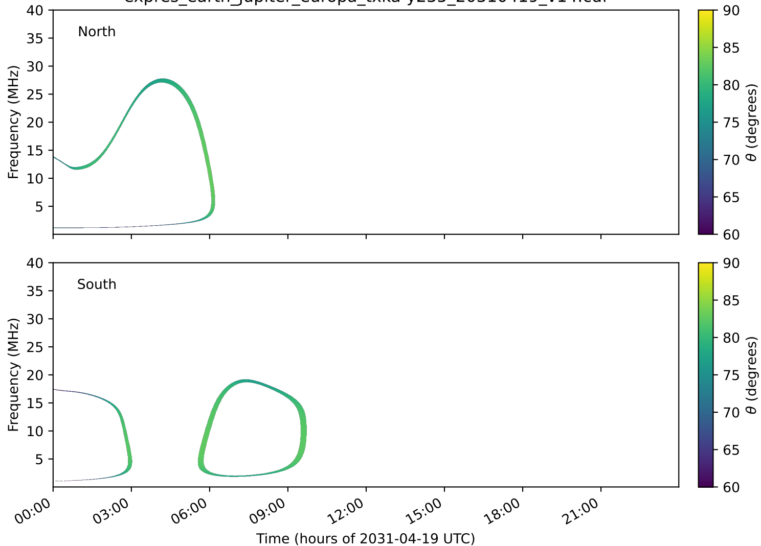
expres_earth_jupiter_europa_txka-y235_20310419_v14.cdf
