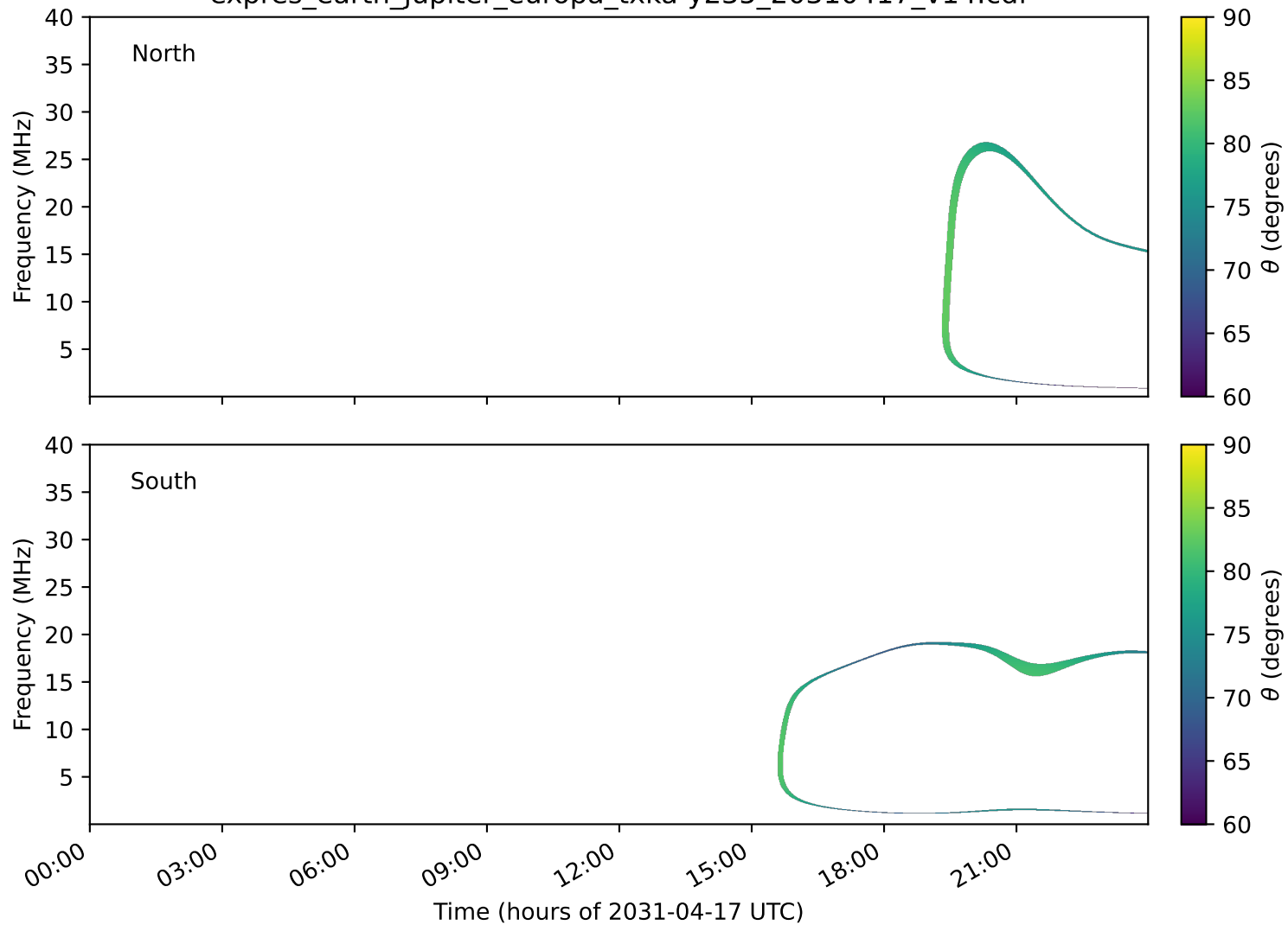
expres_earth_jupiter_europa_txka-y235_20310417_v14.cdf
