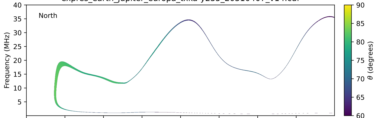
expres_earth_jupiter_europa_txka-y235_20310407_v14.cdf
