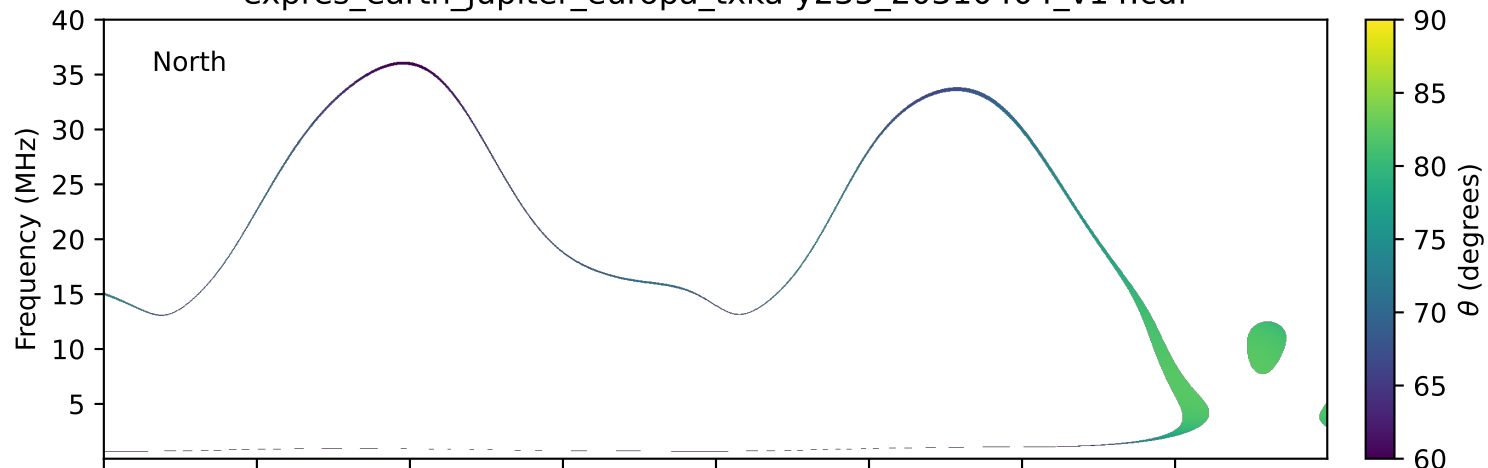
expres_earth_jupiter_europa_txka-y235_20310404_v14.cdf
