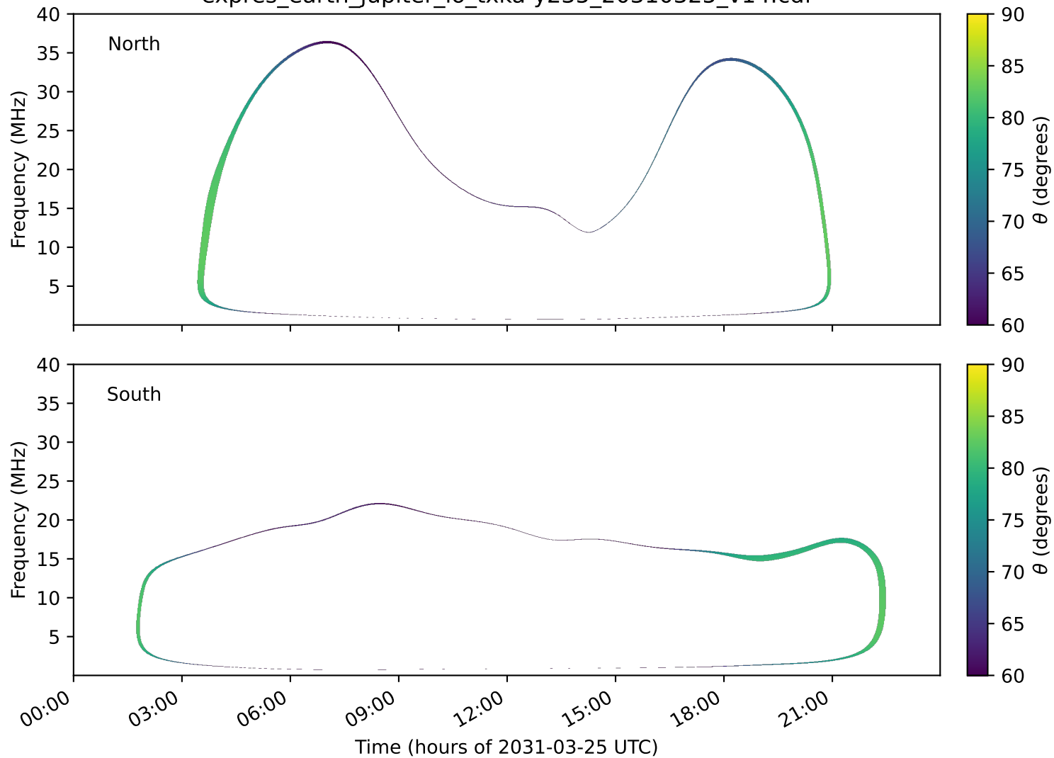
expres_earth_jupiter_io_txka-y235_20310325_v14.cdf
