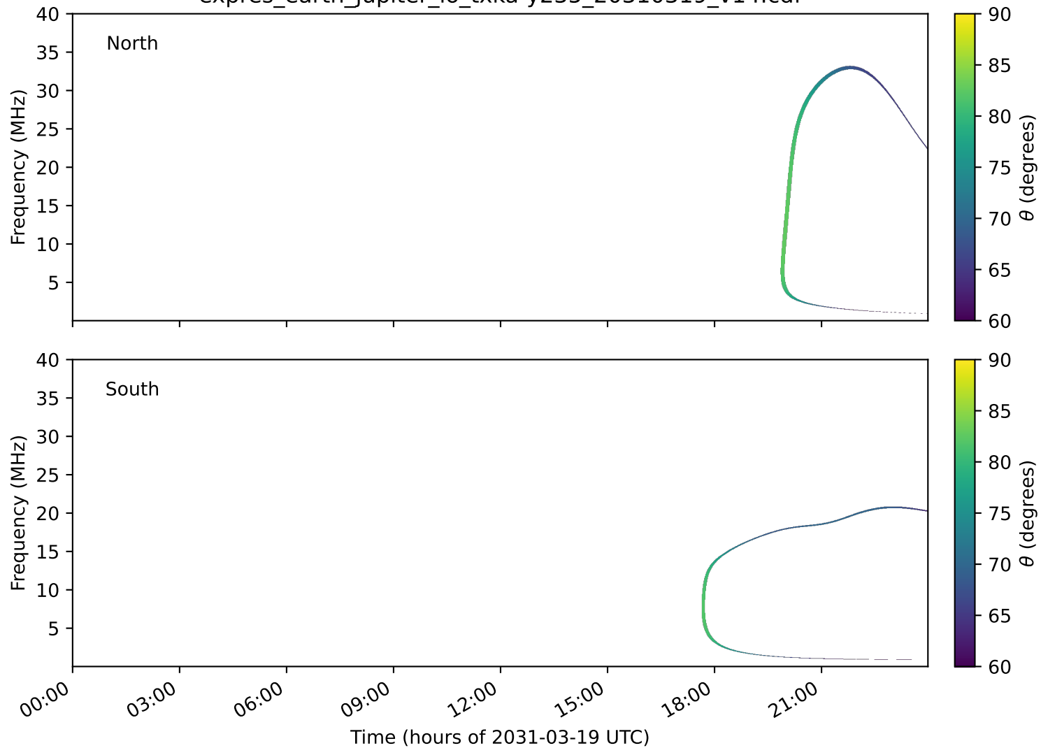
expres_earth_jupiter_io_txka-y235_20310319_v14.cdf
