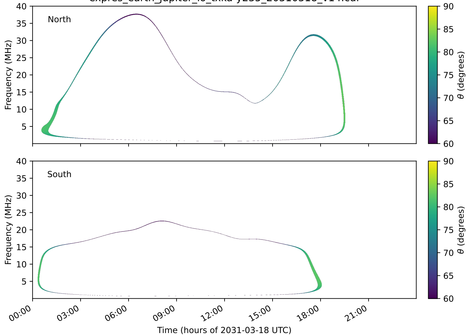
expres_earth_jupiter_io_txka-y235_20310318_v14.cdf
