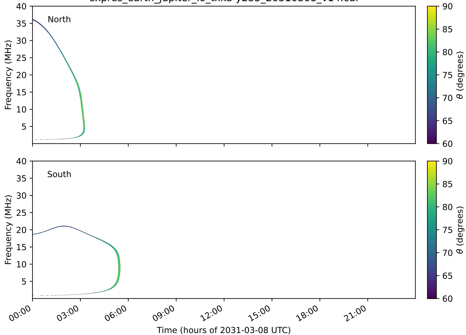
expres_earth_jupiter_io_txka-y235_20310308_v14.cdf
