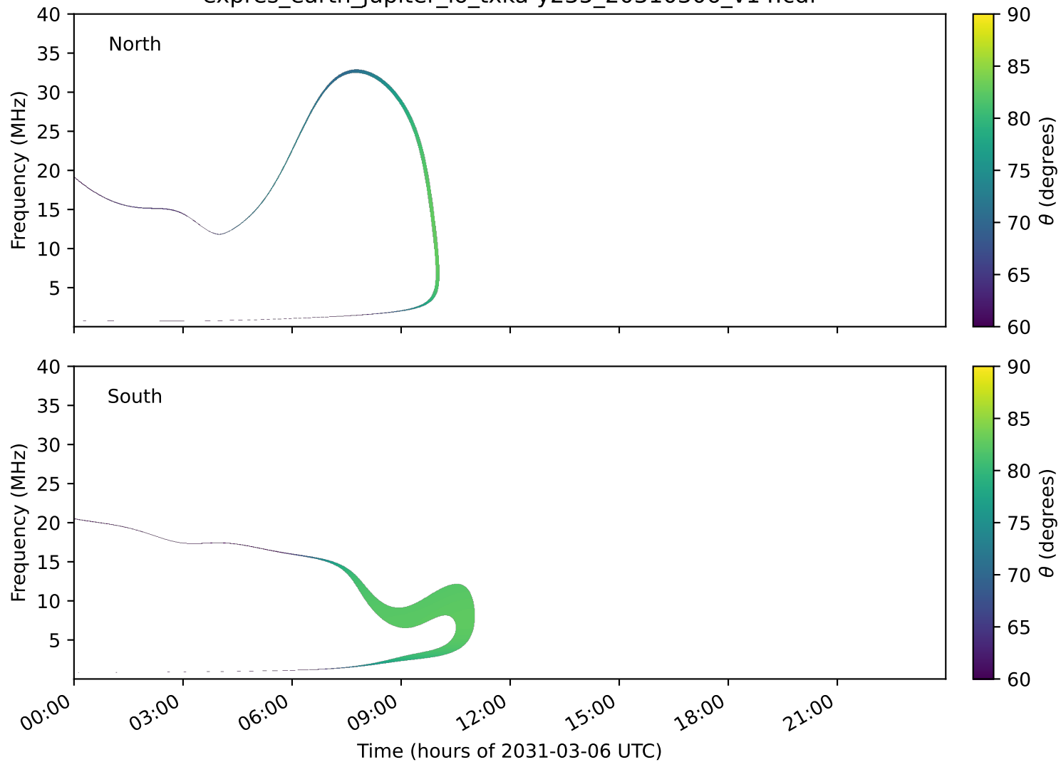
expres_earth_jupiter_io_txka-y235_20310306_v14.cdf
