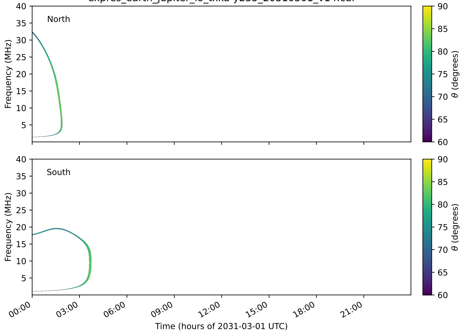
expres_earth_jupiter_io_txka-y235_20310301_v14.cdf
