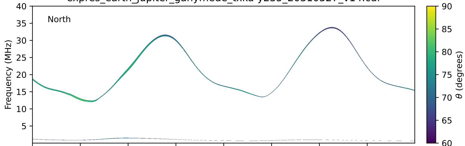
expres_earth_jupiter_ganymede_txka-y235_20310327_v14.cdf
