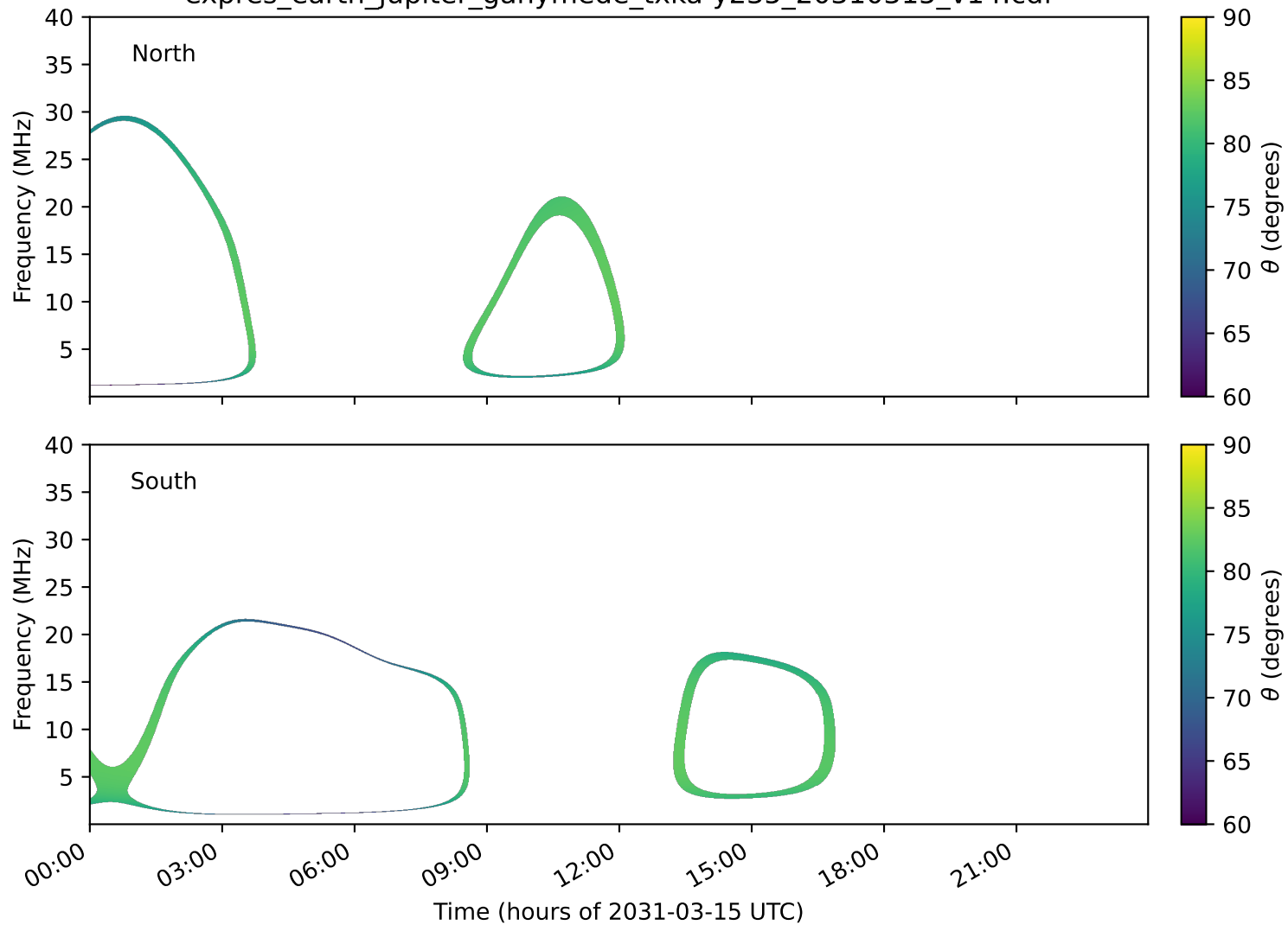
expres_earth_jupiter_ganymede_txka-y235_20310315_v14.cdf
