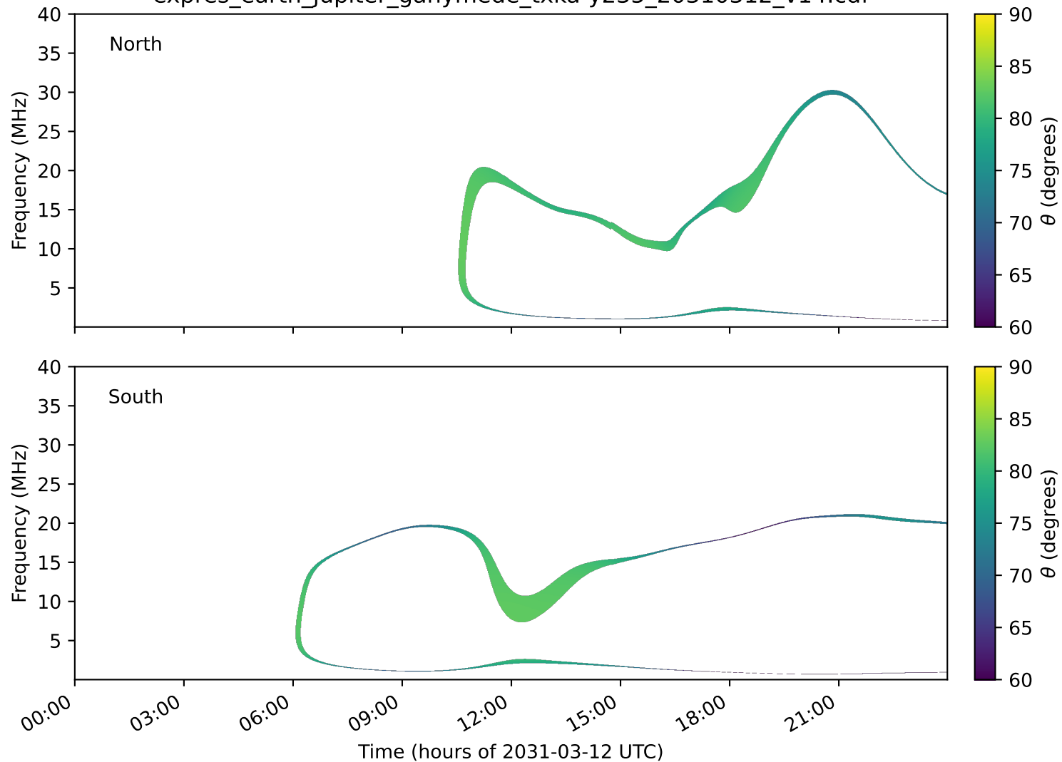
expres_earth_jupiter_ganymede_txka-y235_20310312_v14.cdf
