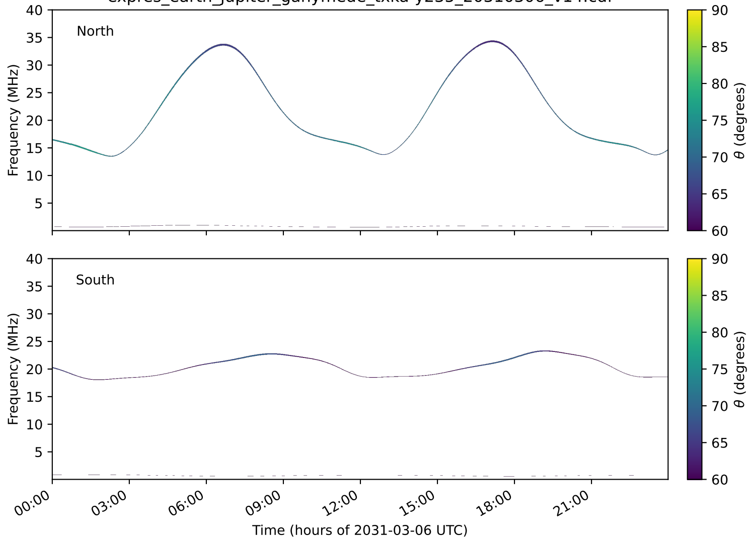
expres_earth_jupiter_ganymede_txka-y235_20310306_v14.cdf
