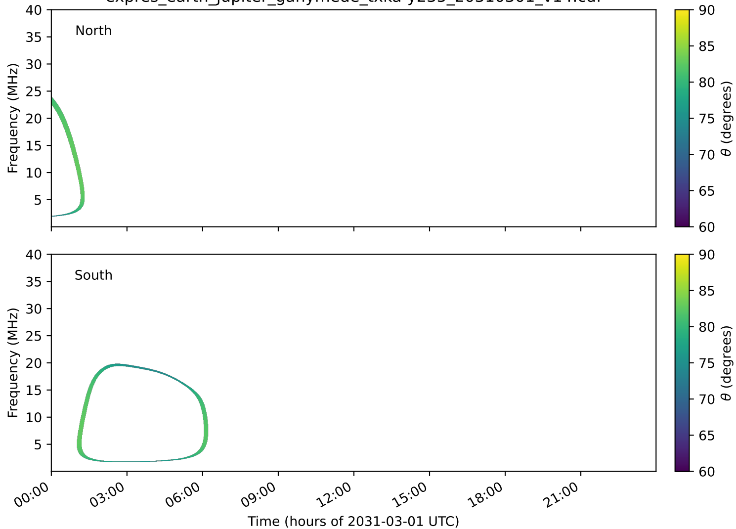
expres_earth_jupiter_ganymede_txka-y235_20310301_v14.cdf
