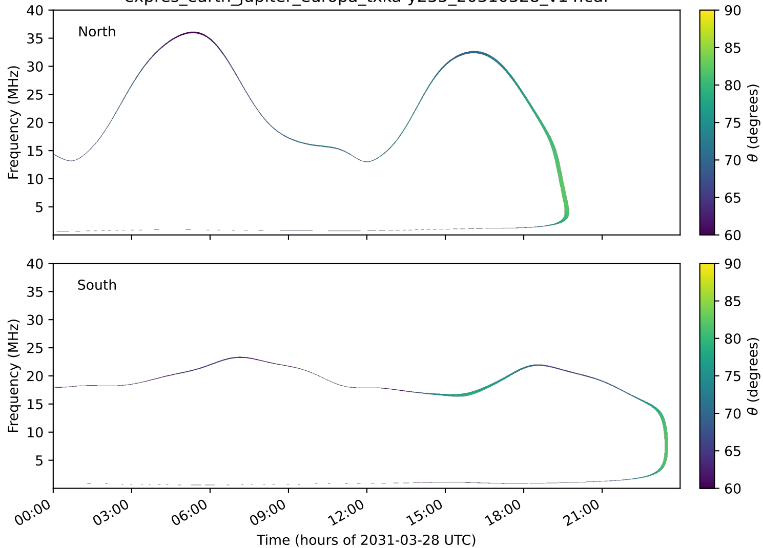
expres_earth_jupiter_europa_txka-y235_20310328_v14.cdf
