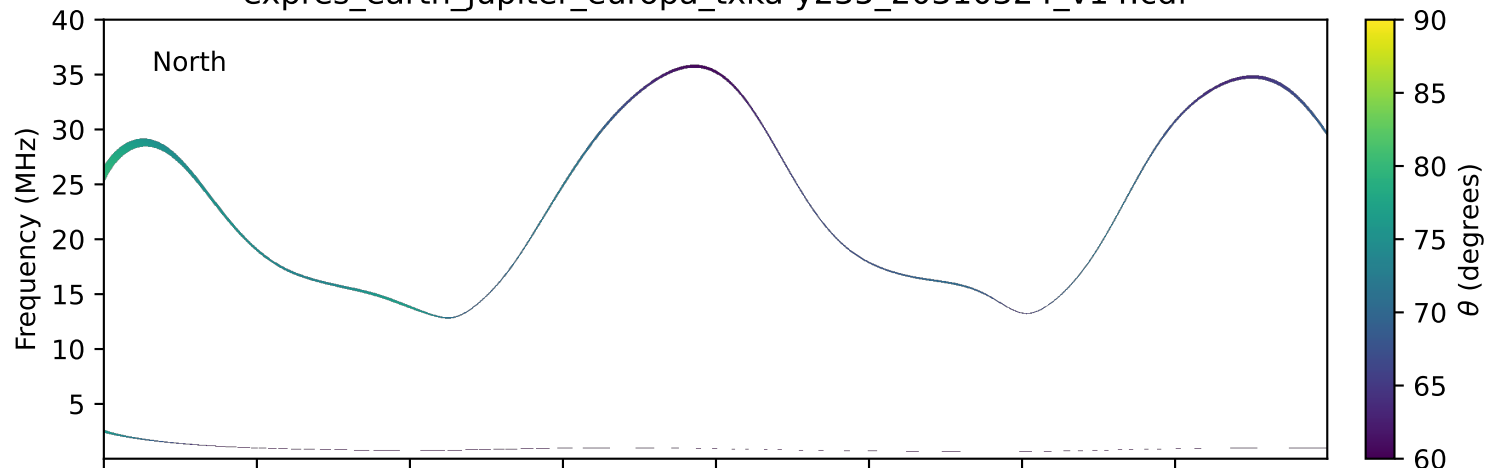
expres_earth_jupiter_europa_txka-y235_20310324_v14.cdf
