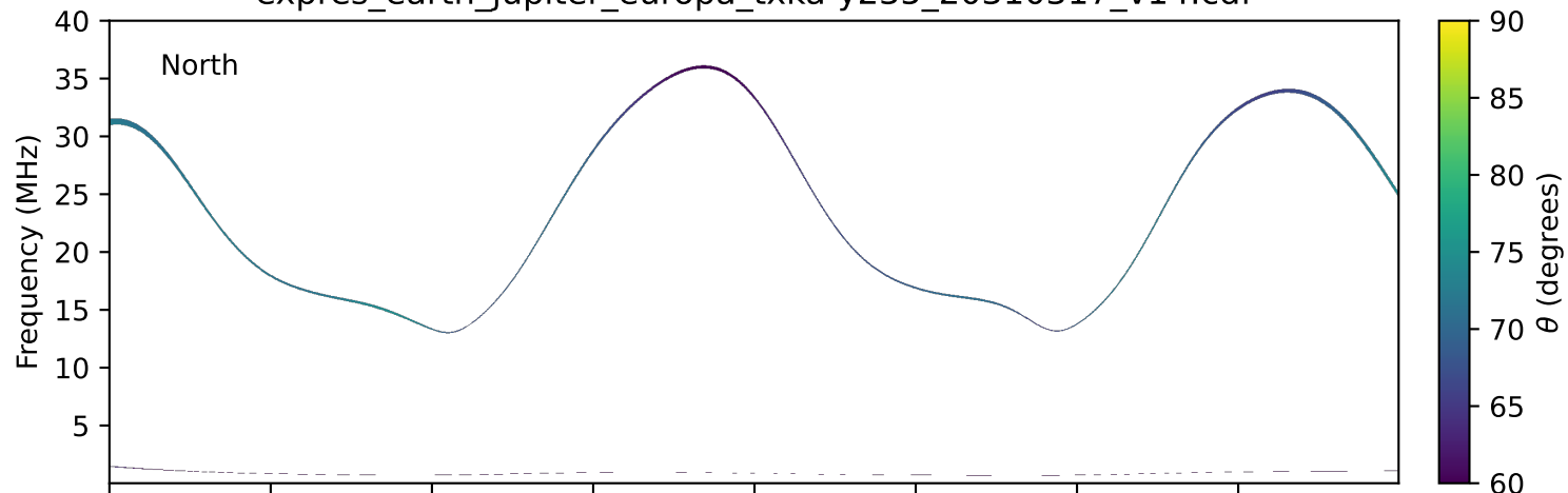
expres_earth_jupiter_europa_txka-y235_20310317_v14.cdf
