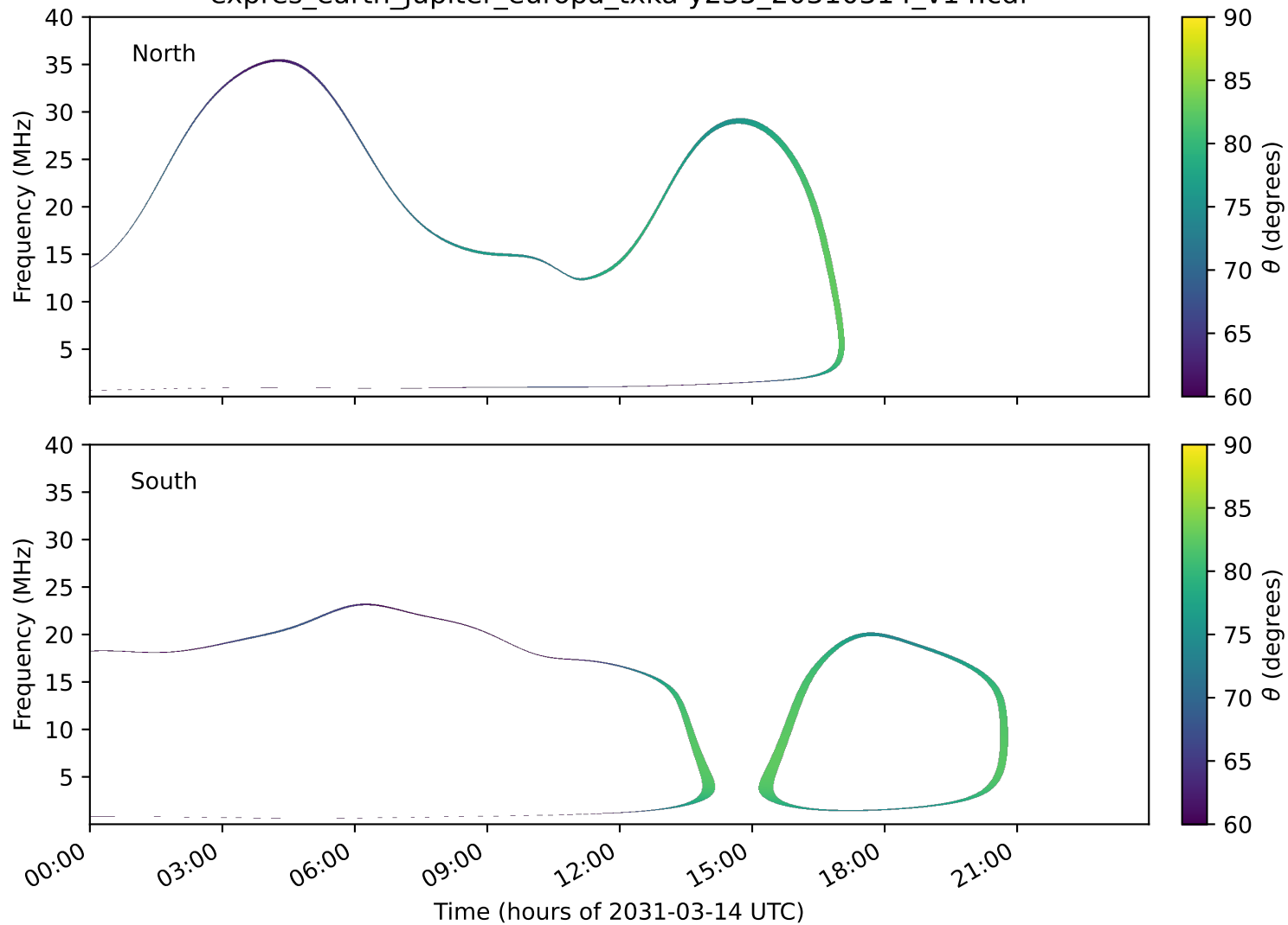
expres_earth_jupiter_europa_txka-y235_20310314_v14.cdf
