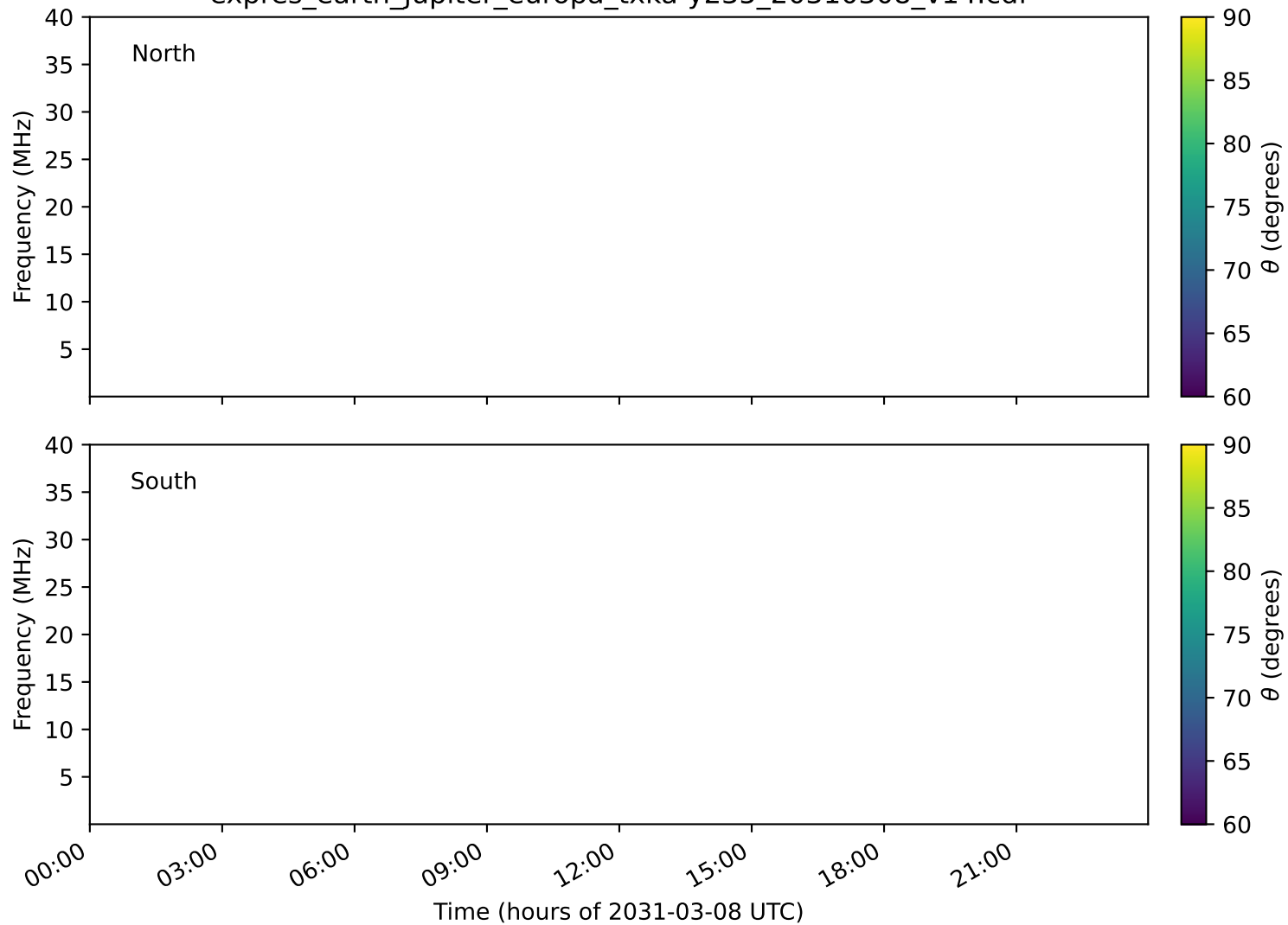
expres_earth_jupiter_europa_txka-y235_20310308_v14.cdf
