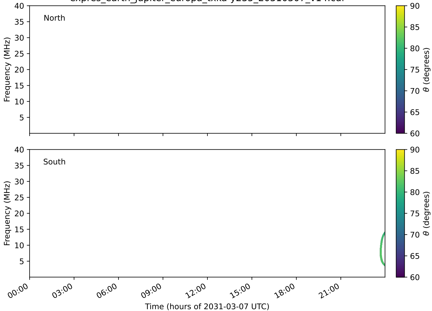
expres_earth_jupiter_europa_txka-y235_20310307_v14.cdf
