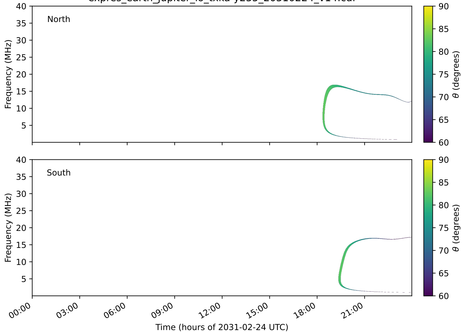
expres_earth_jupiter_io_txka-y235_20310224_v14.cdf
