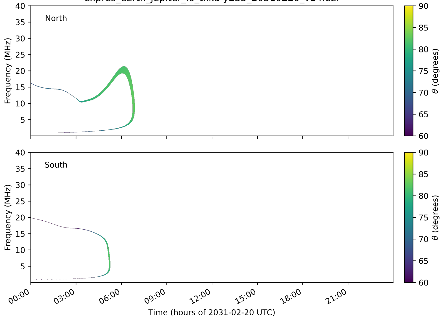
expres_earth_jupiter_io_txka-y235_20310220_v14.cdf
