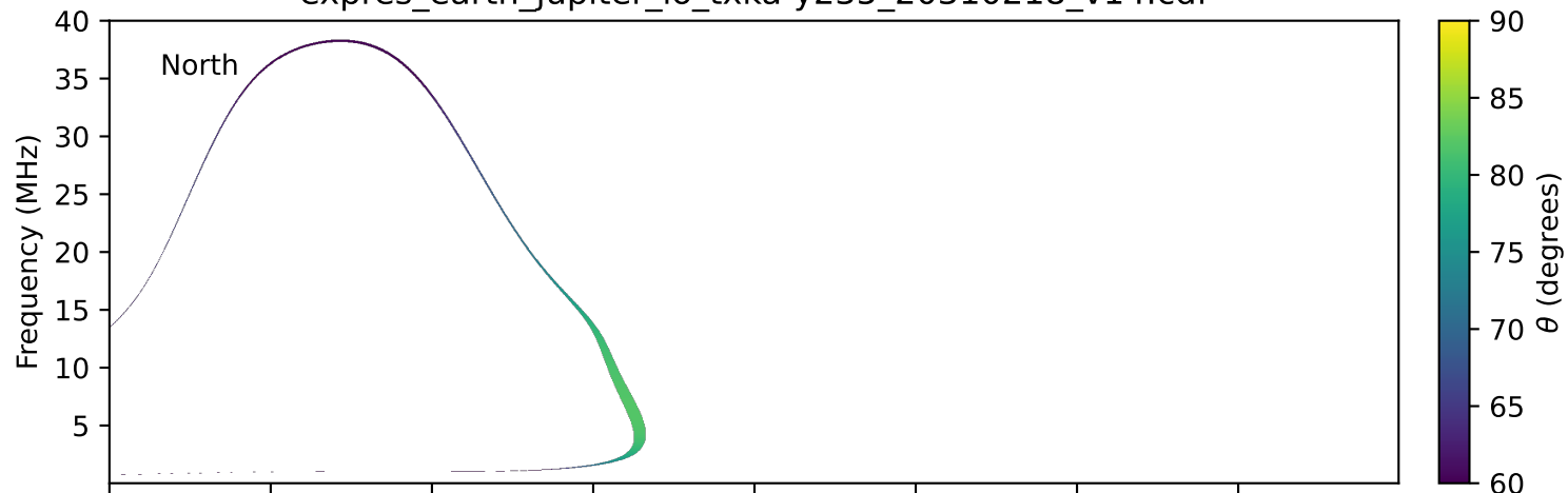
expres_earth_jupiter_io_txka-y235_20310218_v14.cdf
