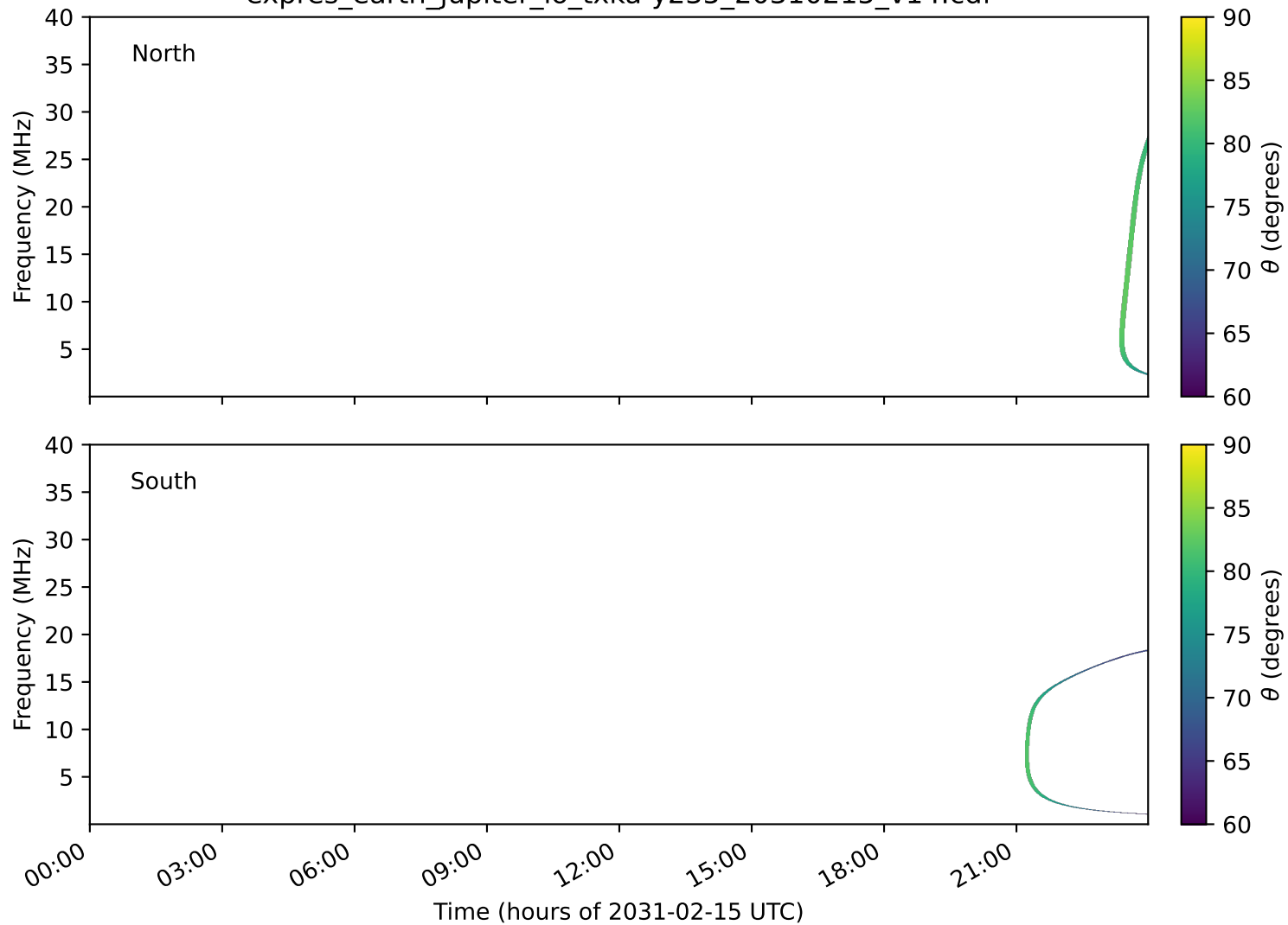
expres_earth_jupiter_io_txka-y235_20310215_v14.cdf
