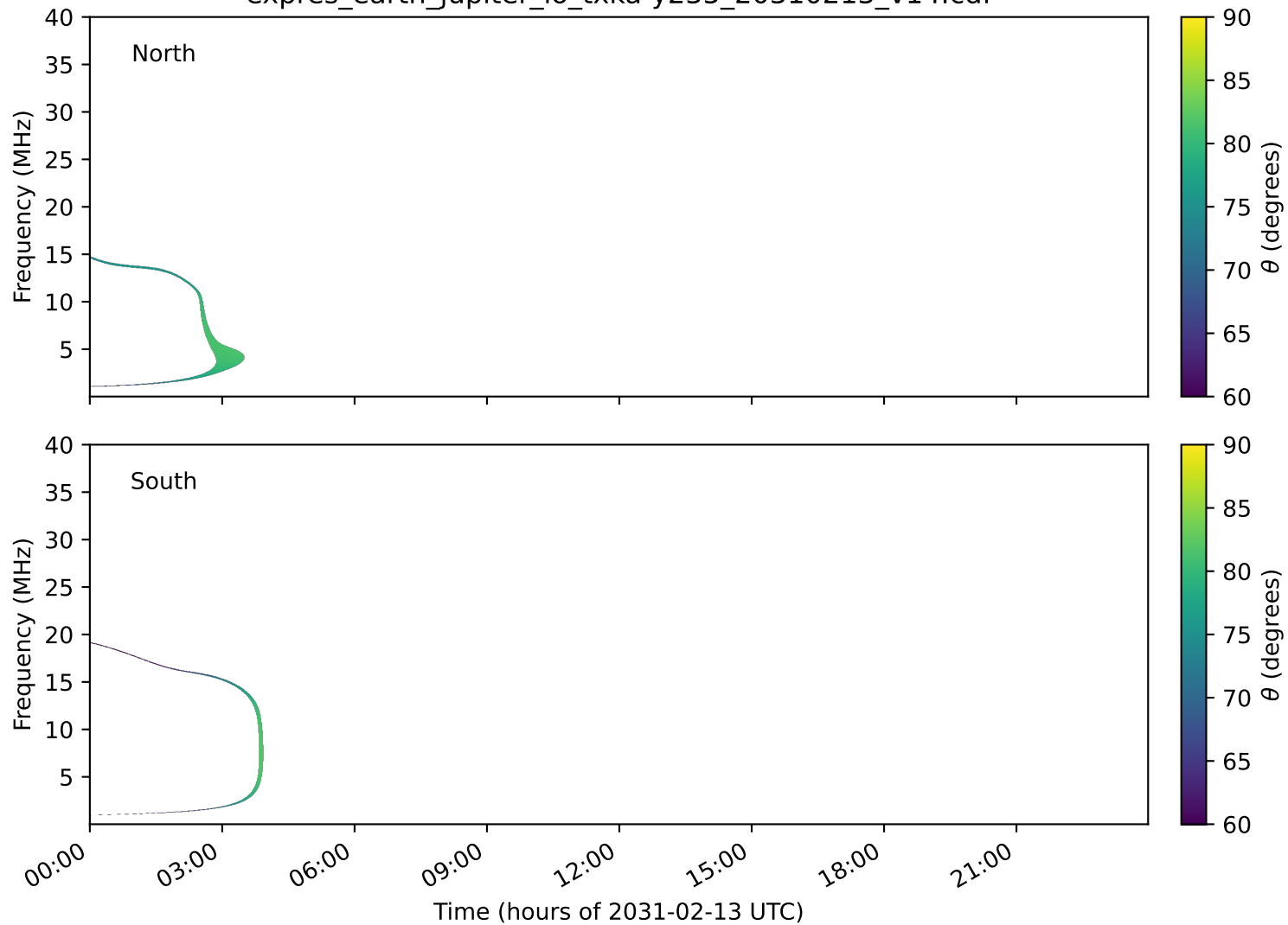
expres_earth_jupiter_io_txka-y235_20310213_v14.cdf
