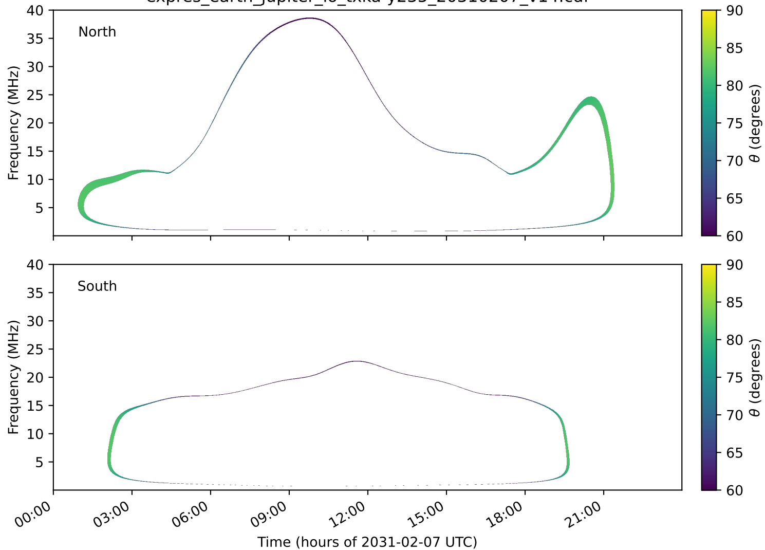
expres_earth_jupiter_io_txka-y235_20310207_v14.cdf
