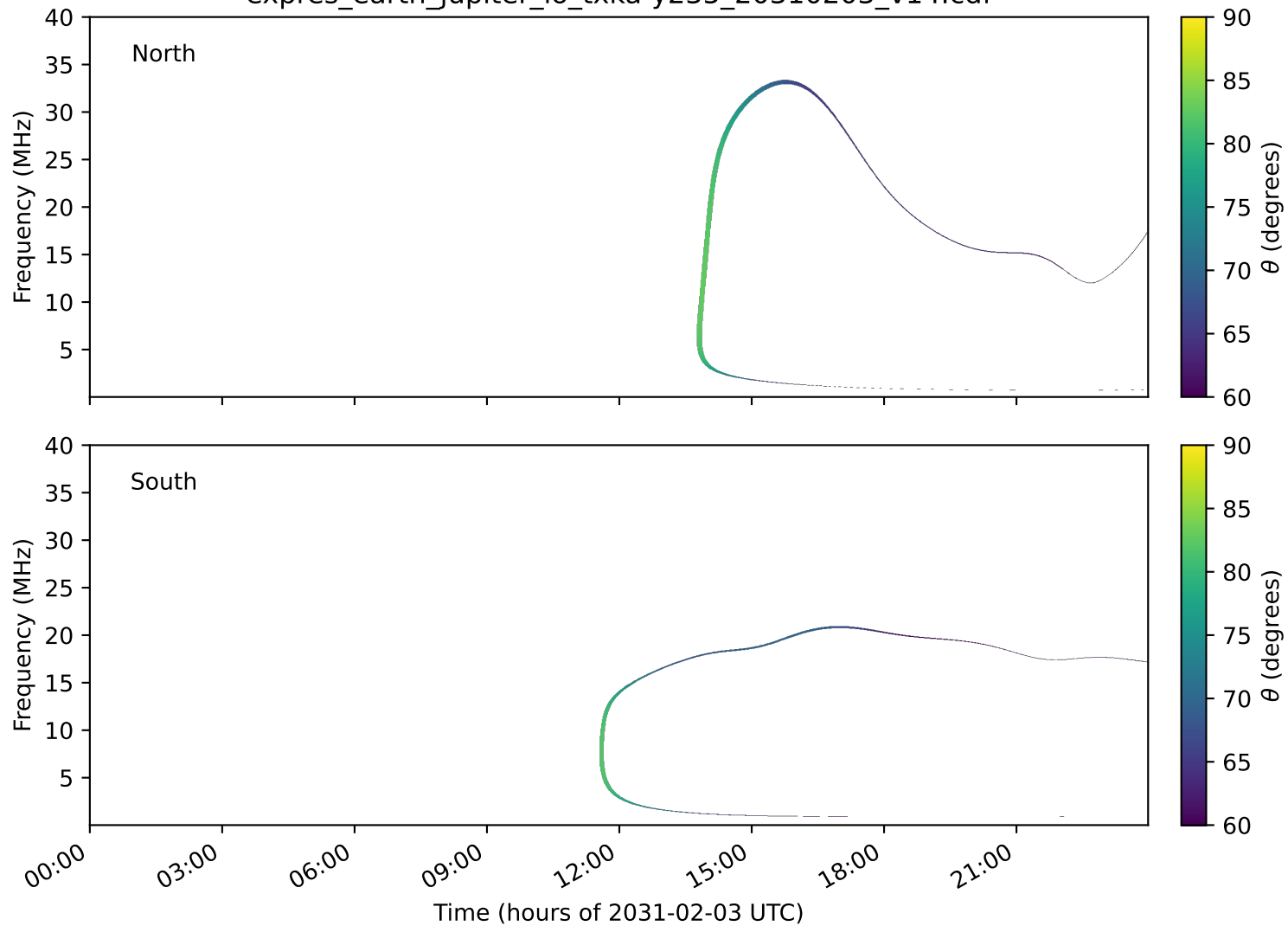
expres_earth_jupiter_io_txka-y235_20310203_v14.cdf
