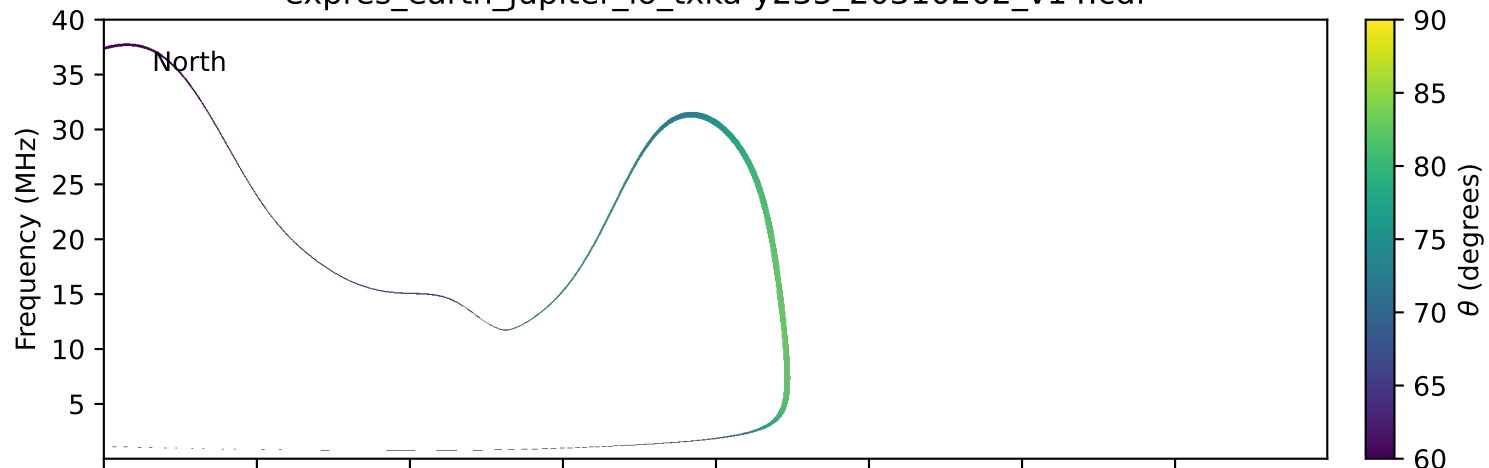
expres_earth_jupiter_io_txka-y235_20310202_v14.cdf
