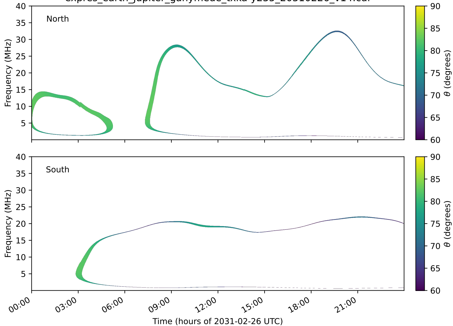
expres_earth_jupiter_ganymede_txka-y235_20310226_v14.cdf
