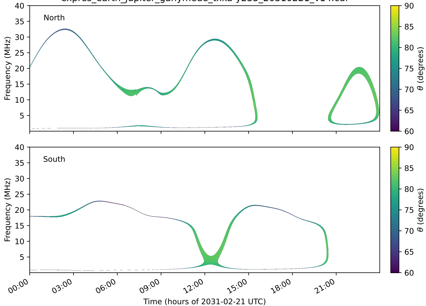
expres_earth_jupiter_ganymede_txka-y235_20310221_v14.cdf
