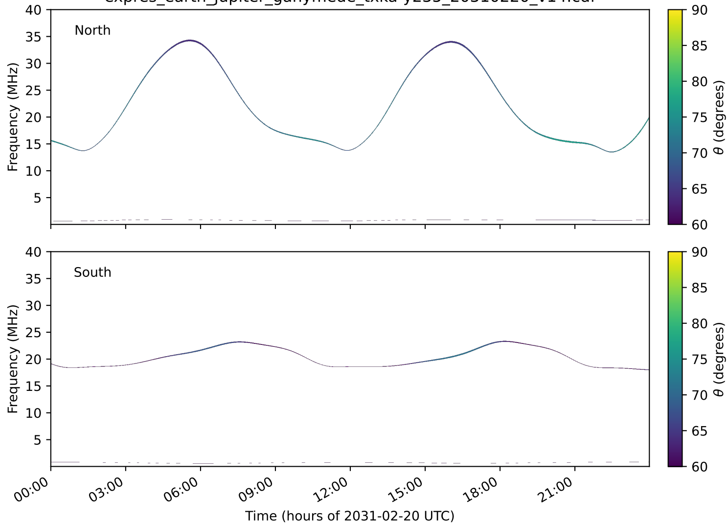
expres_earth_jupiter_ganymede_txka-y235_20310220_v14.cdf
