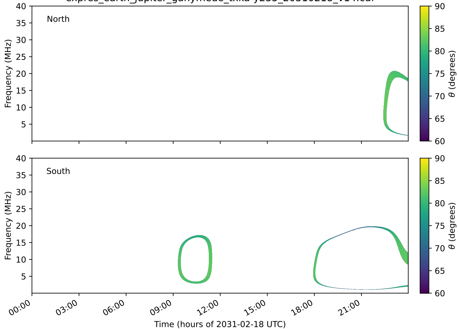
expres_earth_jupiter_ganymede_txka-y235_20310218_v14.cdf
