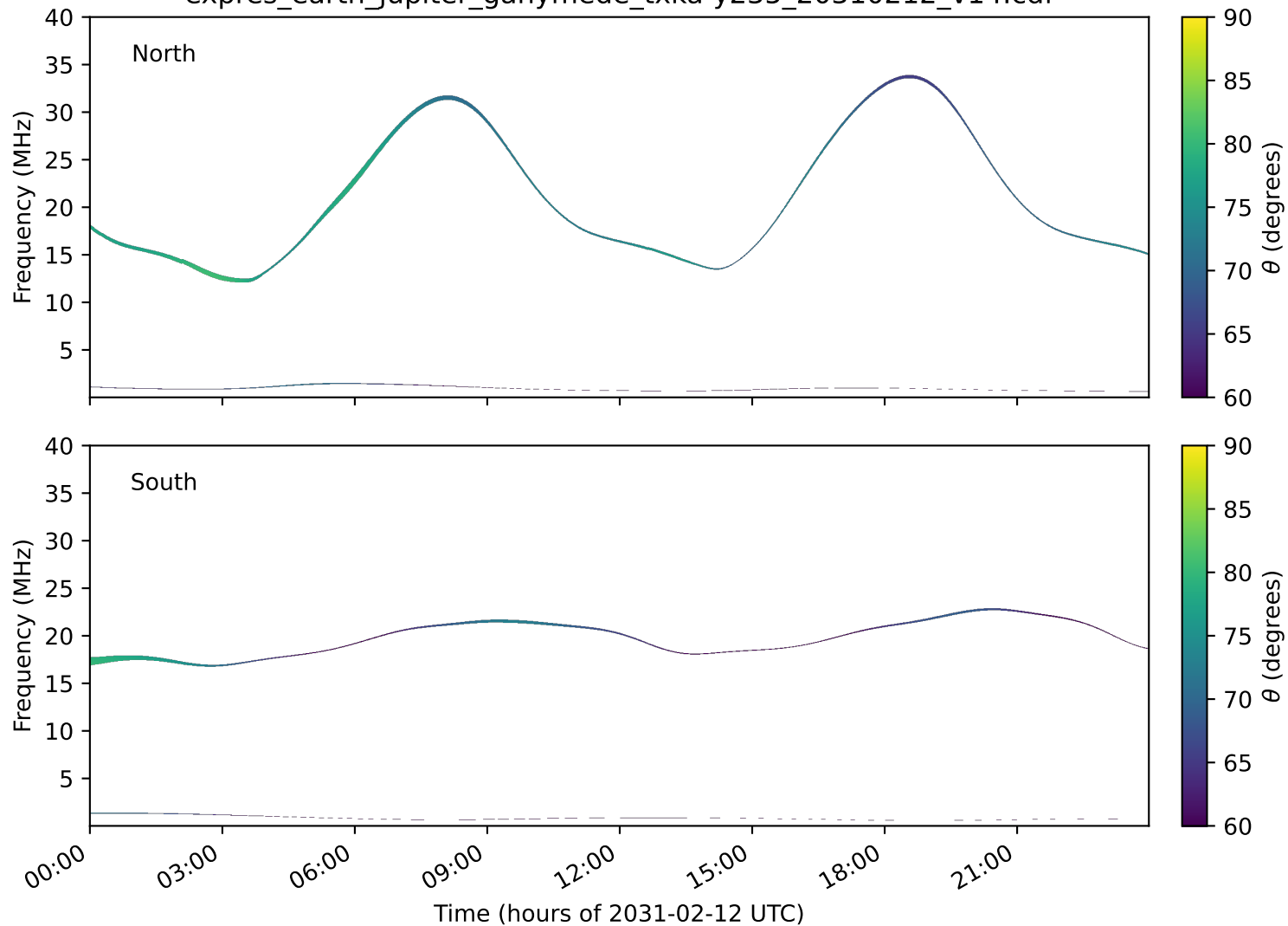
expres_earth_jupiter_ganymede_txka-y235_20310212_v14.cdf
