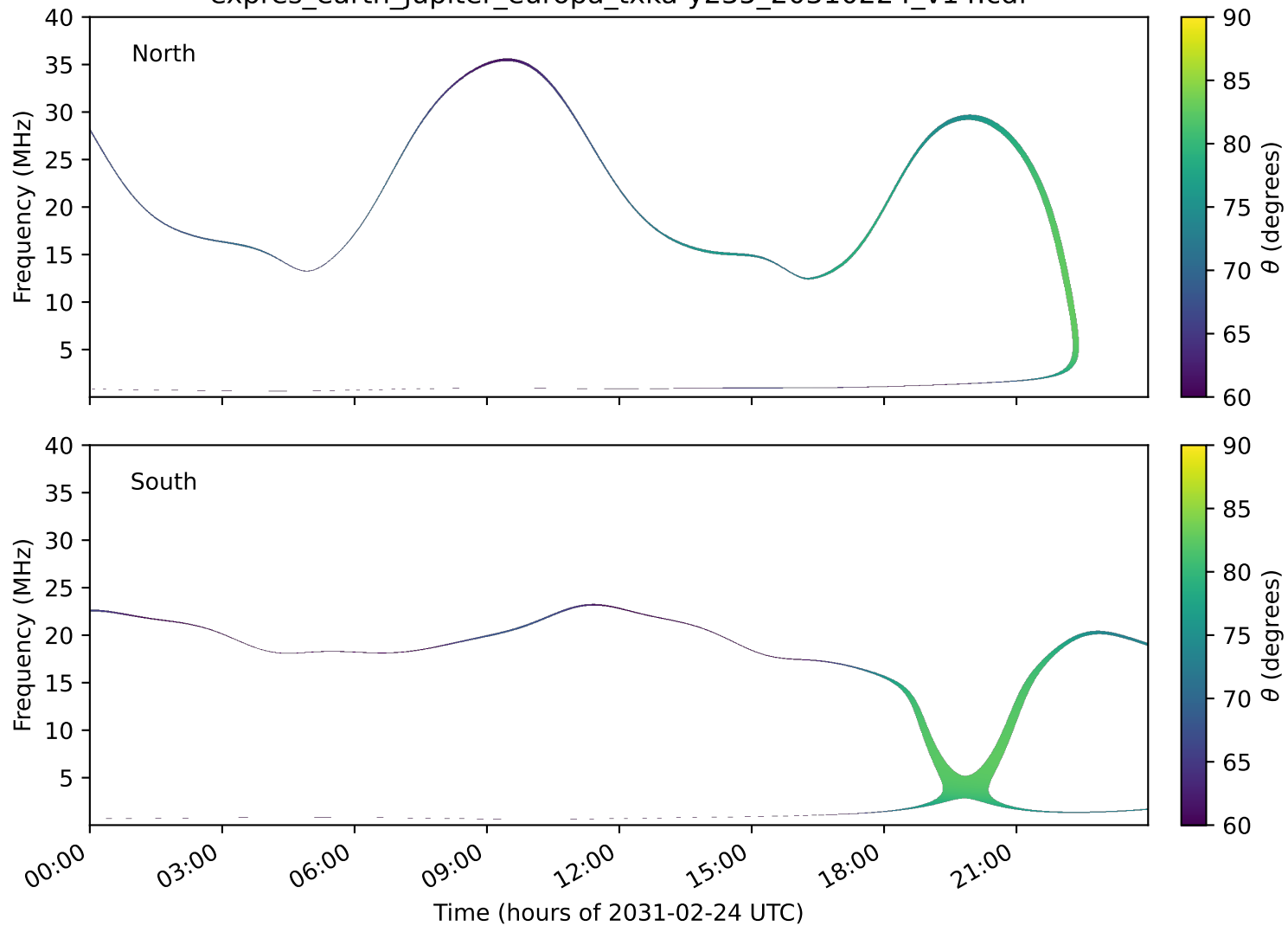
expres_earth_jupiter_europa_txka-y235_20310224_v14.cdf
