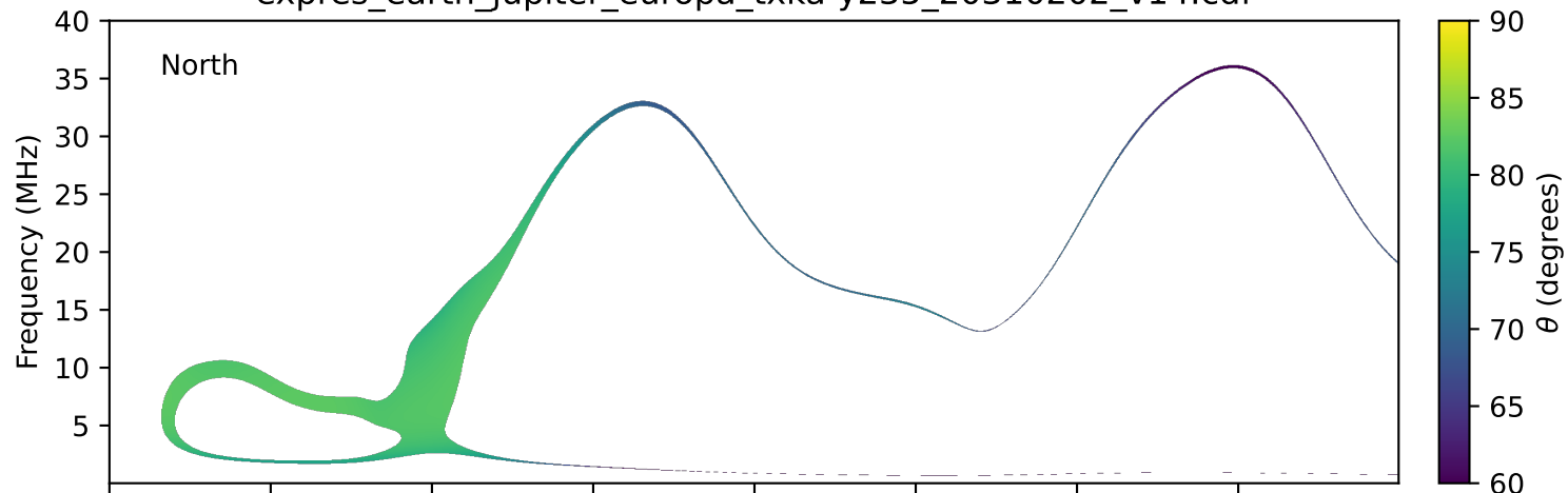
expres_earth_jupiter_europa_txka-y235_20310202_v14.cdf
